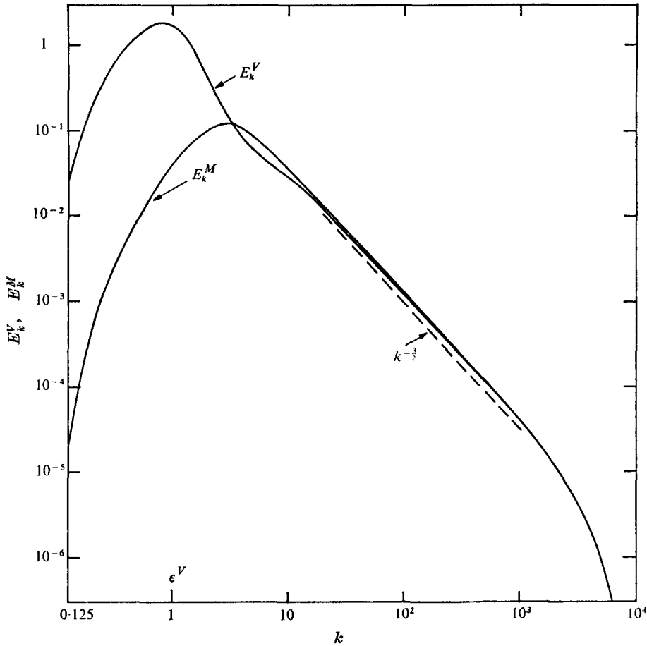
FIGURE 1. The -\frac{3}{2} inertial range of non-helical MHD turbulence. No helicity. V -energy injection spectrum E_k^V = \frac{1}{2}F_k , where F_k = Ck^4 \exp(-2k^2) ( C chosen to give \int_0^\infty F_k dk = 1 ). Initial conditions: E_k^V = 0 , E_k^M = 10^{-3}F_k . Minimum and maximum wavenumbers: 2^{-3} and 2^{14} . Magnetic Prandtl number unity, \nu = \lambda = 10^{-6} . V - and M -energy spectra represented at t = 12 (large-eddy-turnover time of order unity). Notice the slight excess of M -energy in the inertial range.
