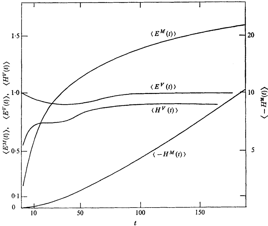
FIGURE 10. Mean V - and M -energies and helicities in the turbulent dynamo. Same conditions as in figure 8. Notice the saturation of V -energy and helicity, but not of M -energy, and the linear growth of M -helicity.
